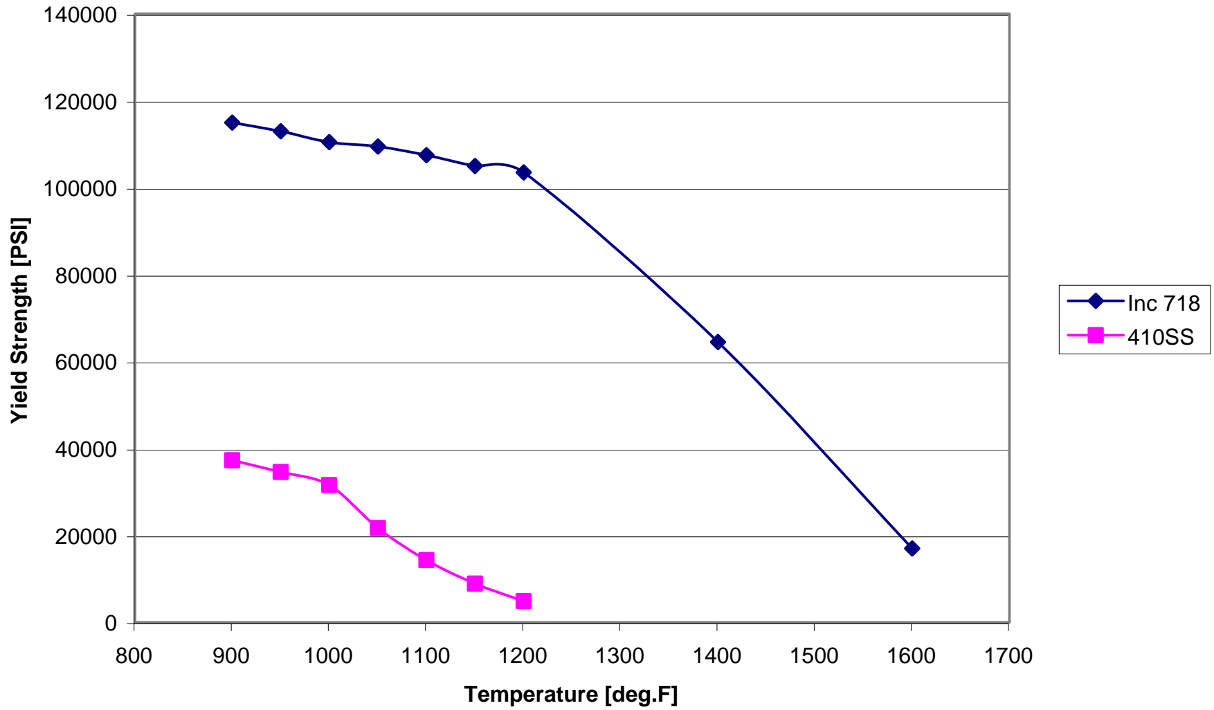
Yield Strength at Elevated Temperature of Inconel 718 Vs 410SS
