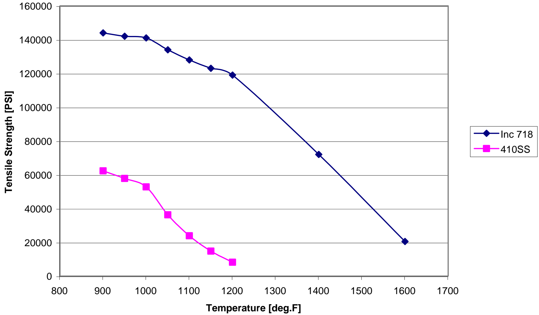
Tensile Strength at Elevated Temperature of Inconel 718 Vs 410SS
